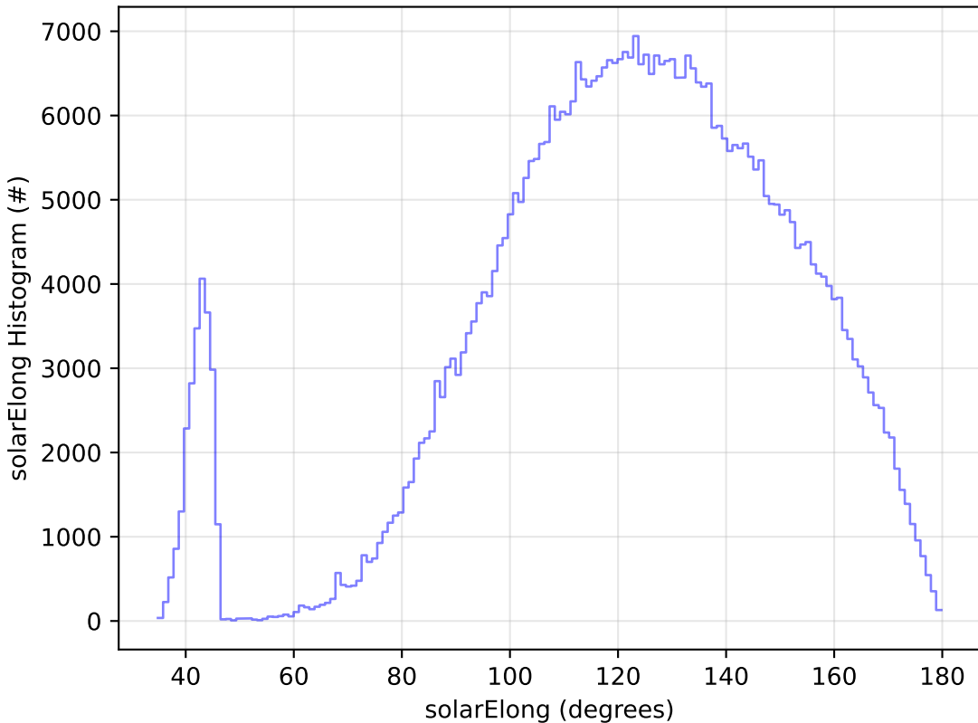
noroll_v3.4_10yrs WFD i band: solarElong Histogram
