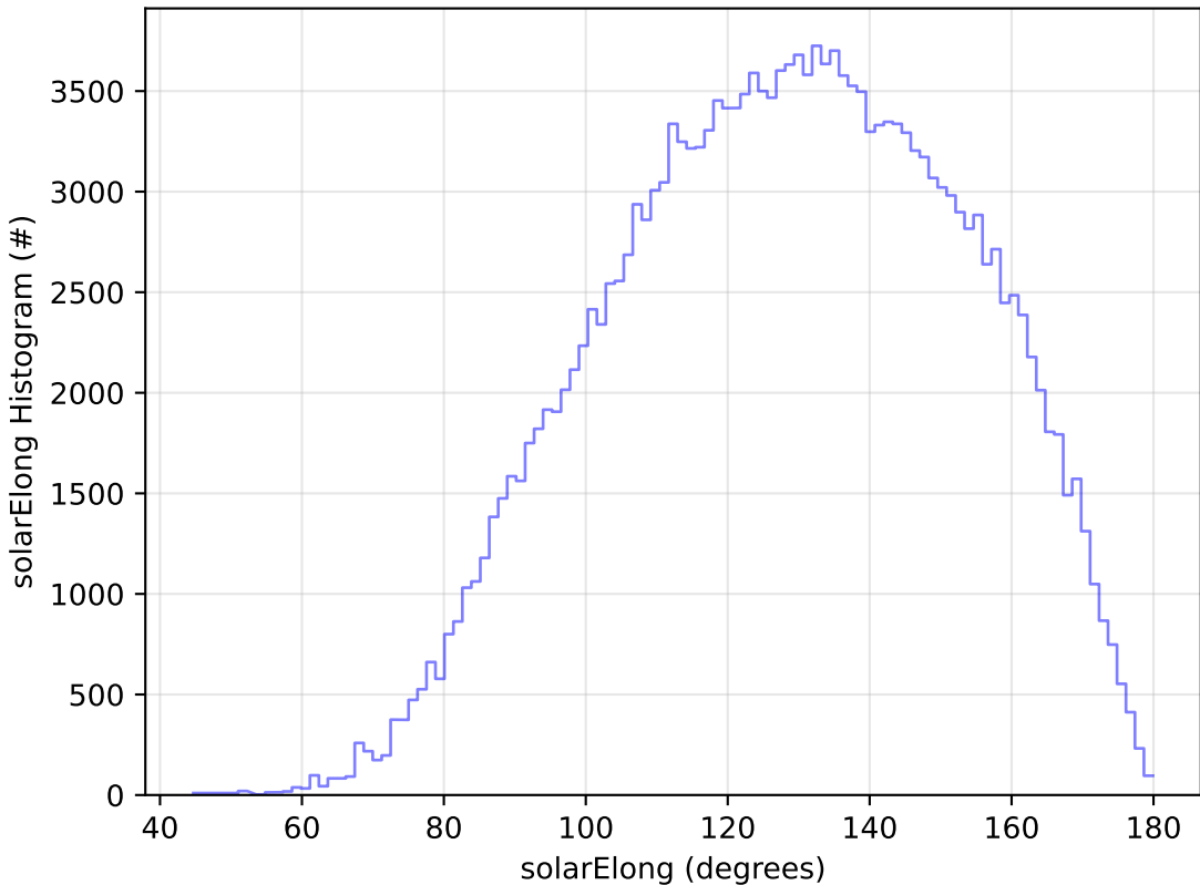
noroll_v3.4_10yrs WFD g band: solarElong Histogram
