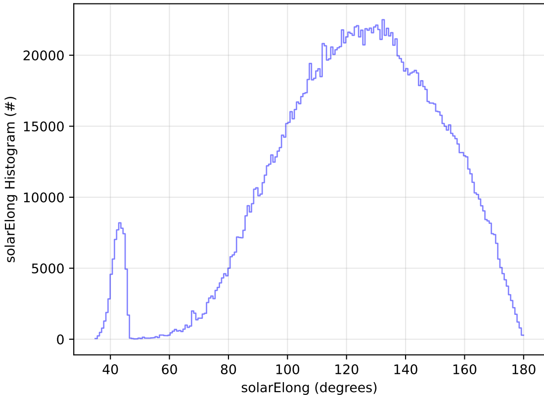
noroll_v3.4_10yrs WFD all bands: solarElong Histogram
