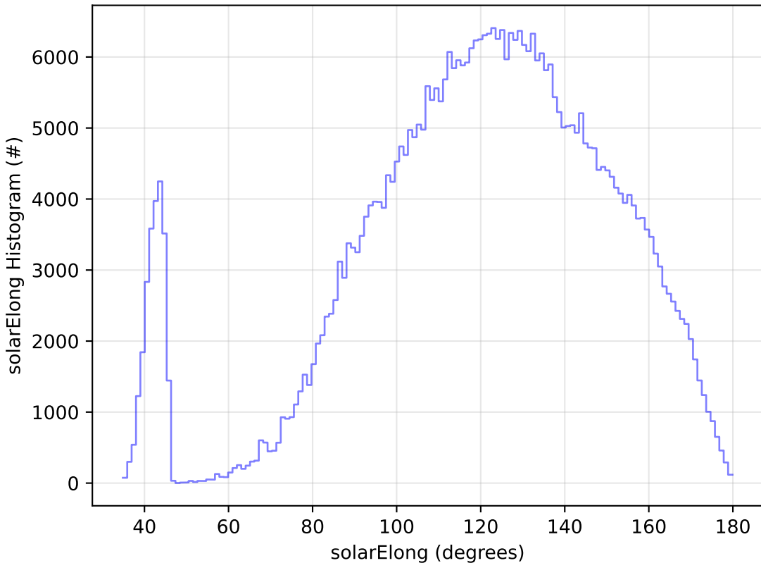
noroll_v3.4_10yrs All sky z band: solarElong Histogram
