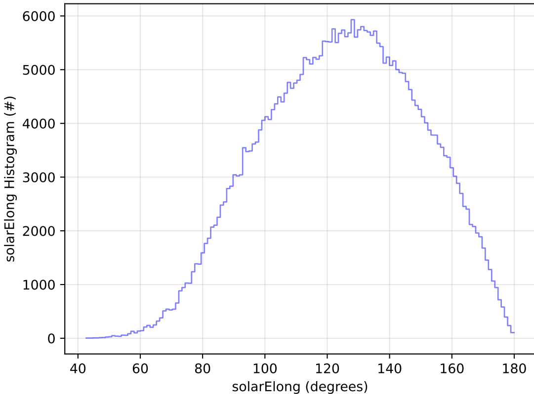
noroll_v3.4_10yrs All sky y band: solarElong Histogram
