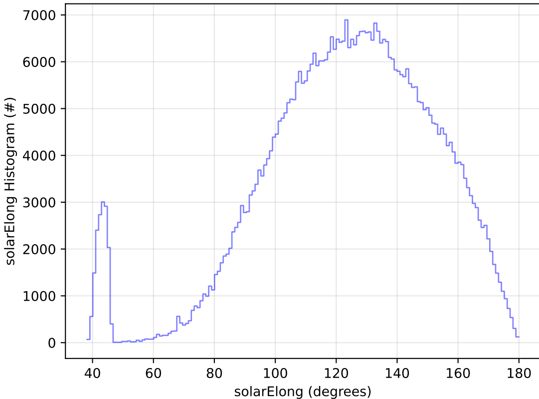
noroll_v3.4_10yrs All sky r band: solarElong Histogram
