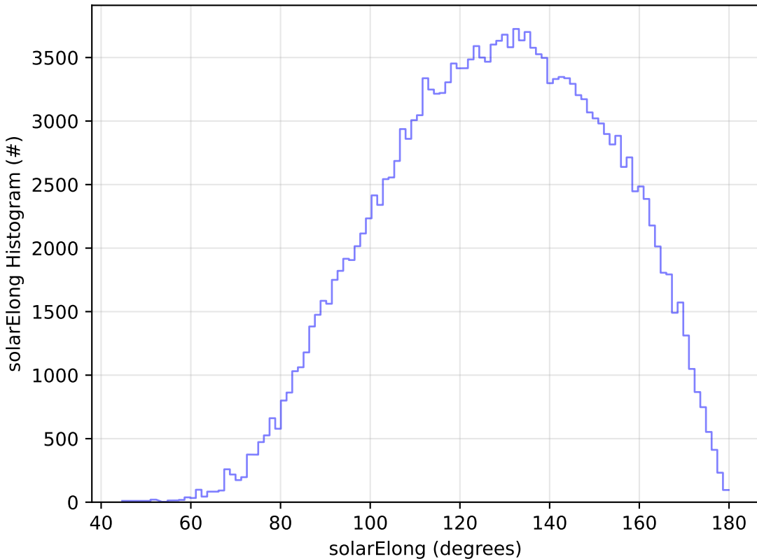
noroll_v3.4_10yrs All sky g band: solarElong Histogram
