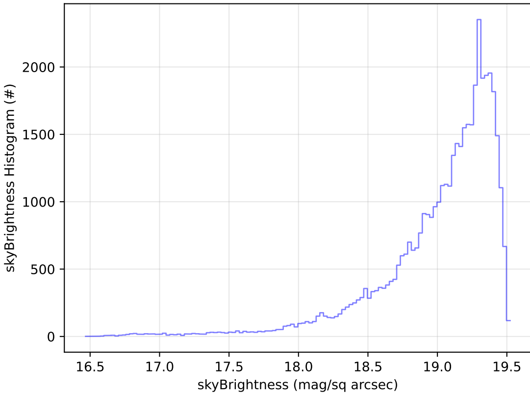
noroll_v3.4_10yrs Yr 1 z band: skyBrightness Histogram
