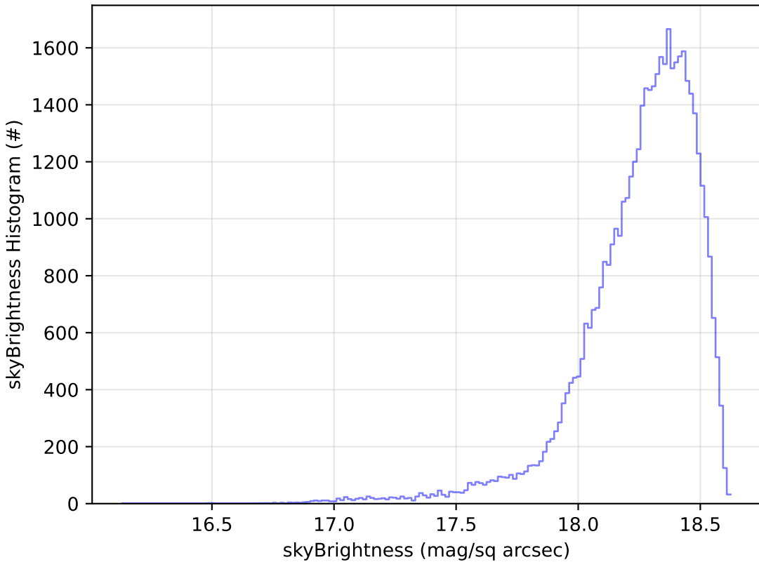
noroll_v3.4_10yrs Yr 1 y band: skyBrightness Histogram
