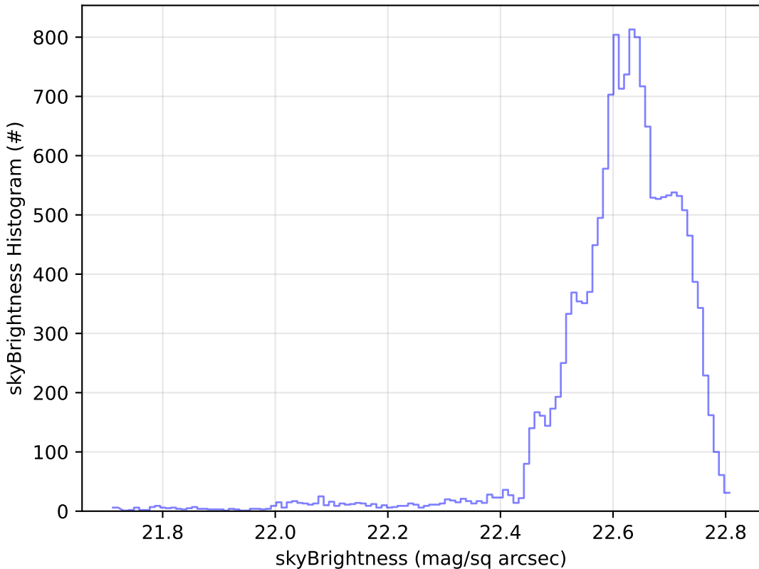
noroll_v3.4_10yrs Yr 1 u band: skyBrightness Histogram
