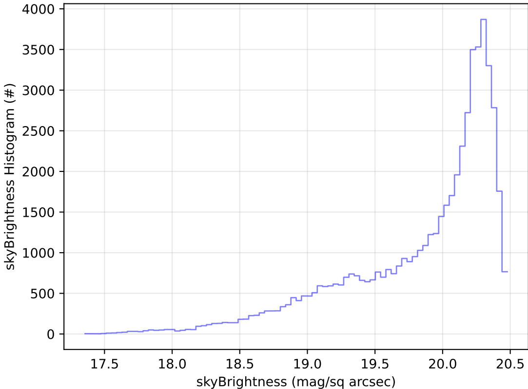
noroll_v3.4_10yrs Yr 1 i band: skyBrightness Histogram
