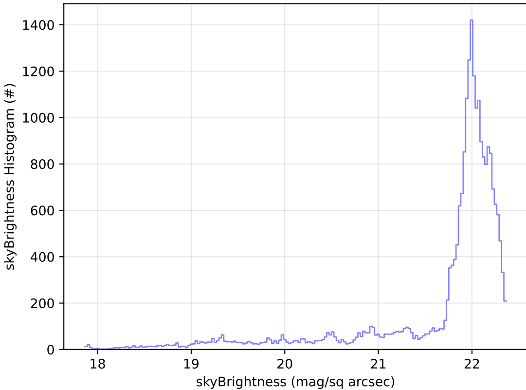
noroll_v3.4_10yrs Yr 1 g band: skyBrightness Histogram
