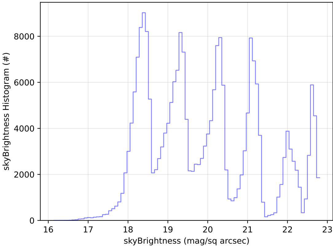
noroll_v3.4_10yrs Yr 1 all bands: skyBrightness Histogram
