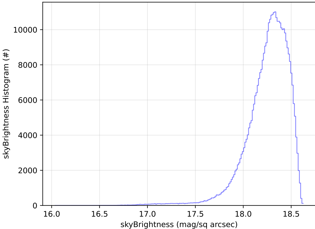
noroll_v3.4_10yrs WFD y band: skyBrightness Histogram
