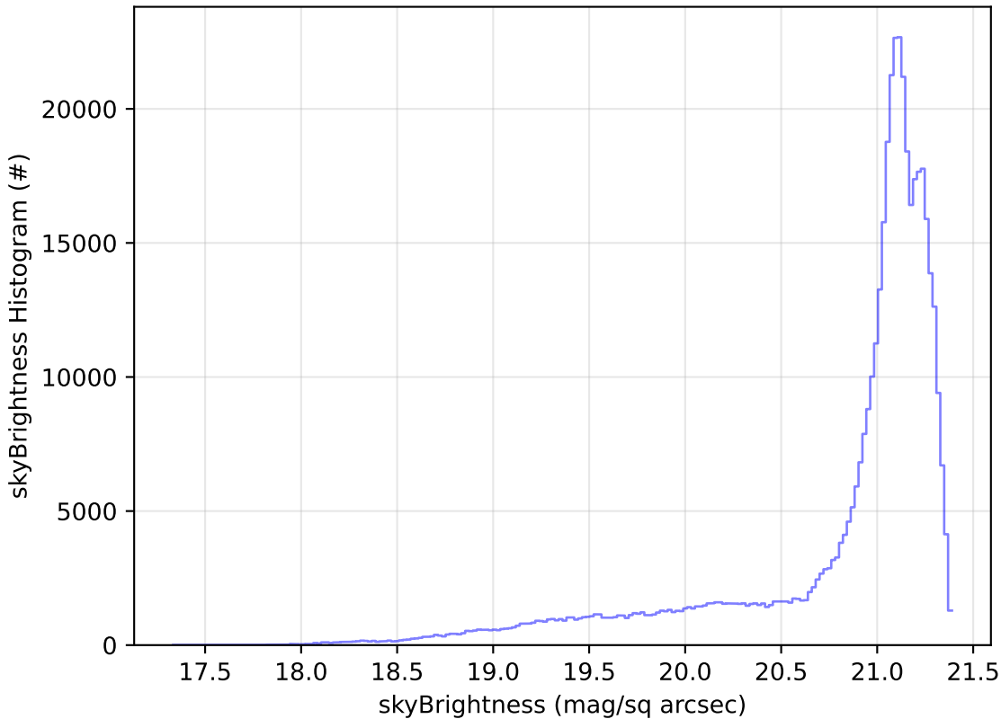
noroll_v3.4_10yrs WFD r band: skyBrightness Histogram
