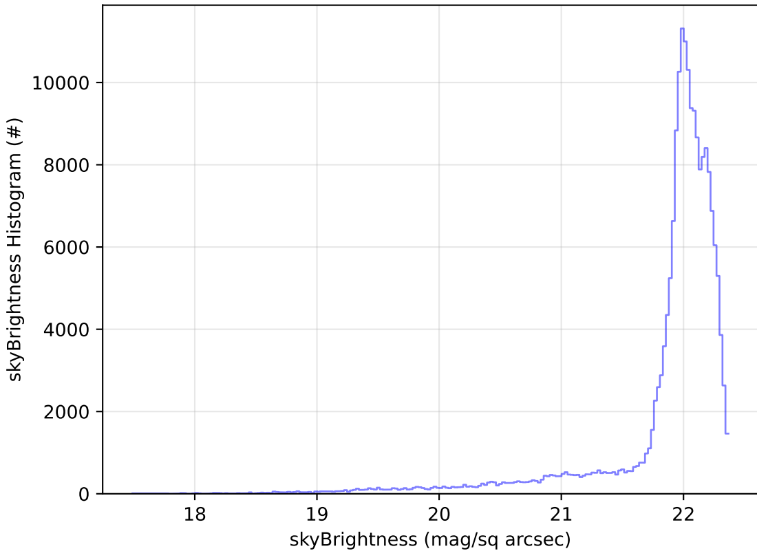
noroll_v3.4_10yrs WFD g band: skyBrightness Histogram
