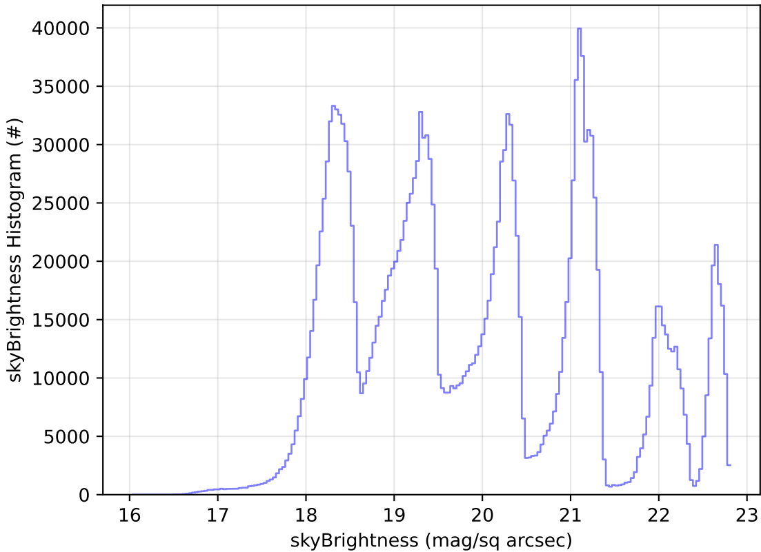
noroll_v3.4_10yrs WFD all bands: skyBrightness Histogram
