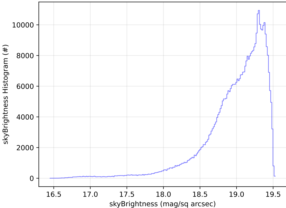
noroll_v3.4_10yrs All sky z band: skyBrightness Histogram
