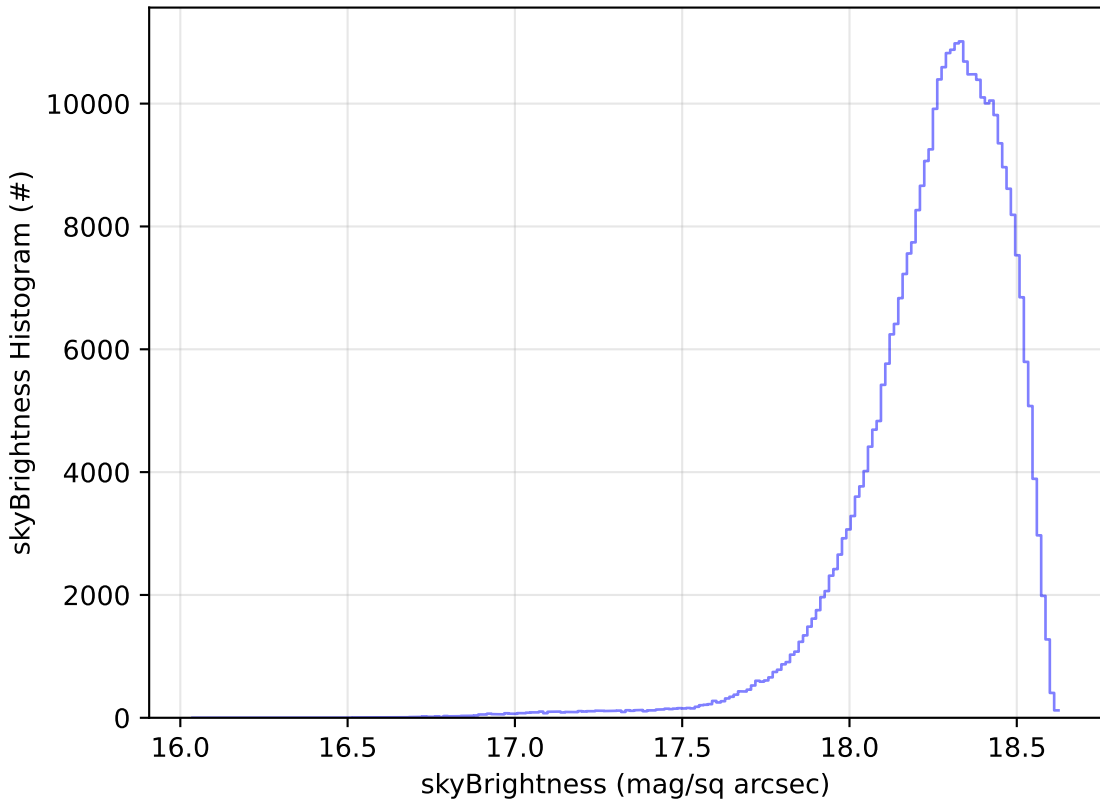
noroll_v3.4_10yrs All sky y band: skyBrightness Histogram
