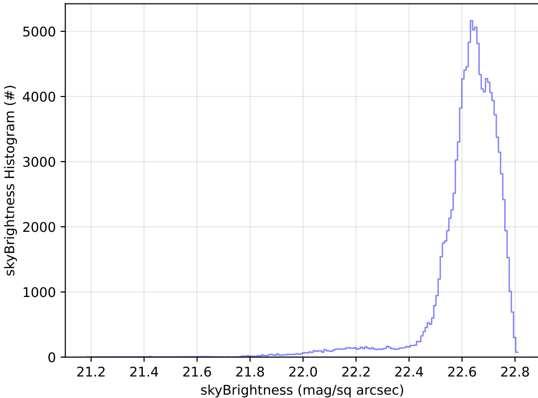
noroll_v3.4_10yrs All sky u band: skyBrightness Histogram
