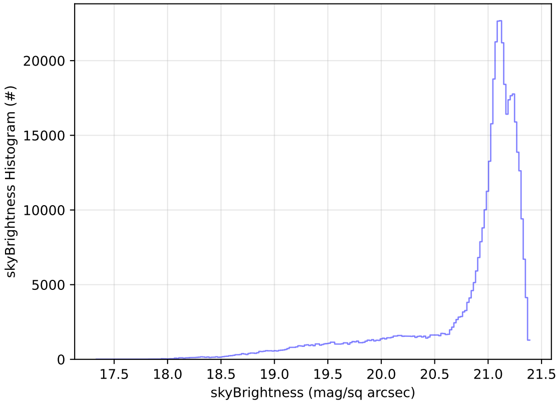
noroll_v3.4_10yrs All sky r band: skyBrightness Histogram
