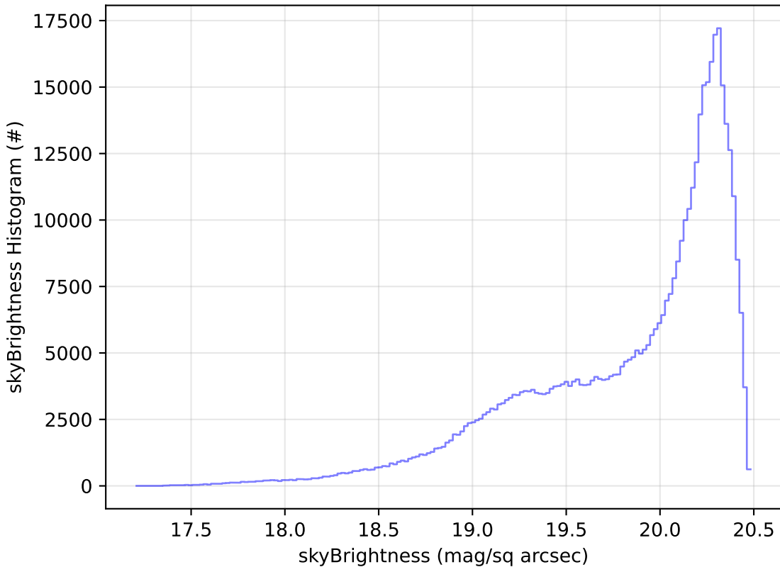
noroll_v3.4_10yrs All sky i band: skyBrightness Histogram
