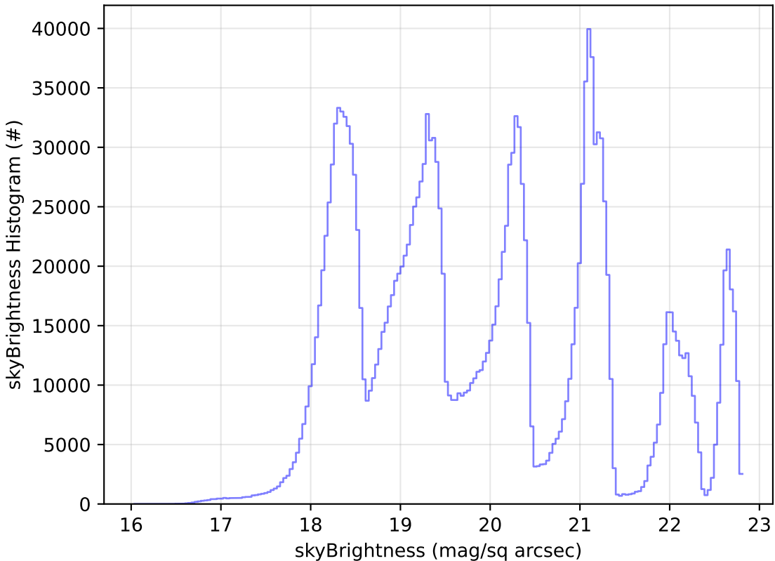
noroll_v3.4_10yrs All sky all bands: skyBrightness Histogram
