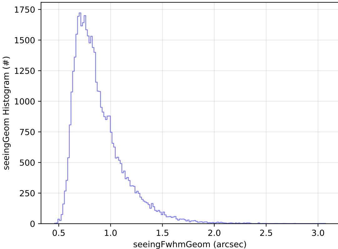
noroll_v3.4_10yrs Yr 1 z band: seeingGeom Histogram
