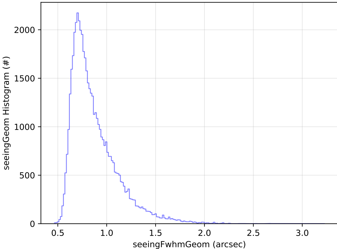
noroll_v3.4_10yrs Yr 1 r band: seeingGeom Histogram
