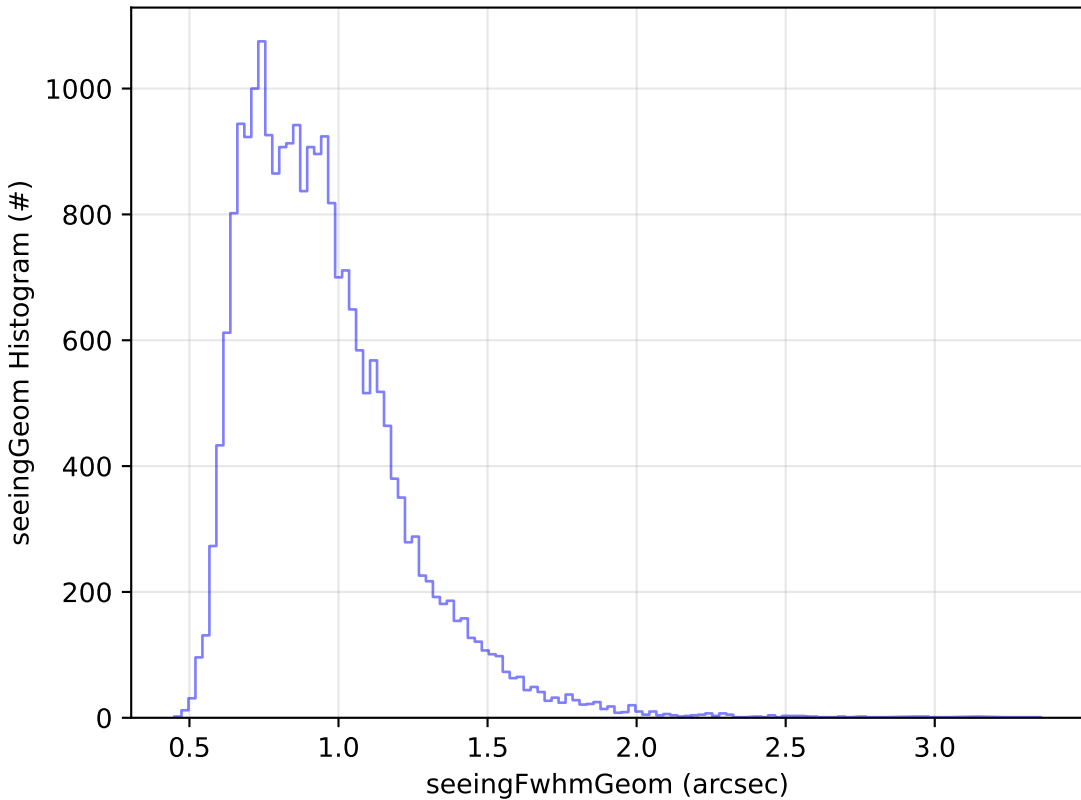
noroll_v3.4_10yrs Yr 1 g band: seeingGeom Histogram
