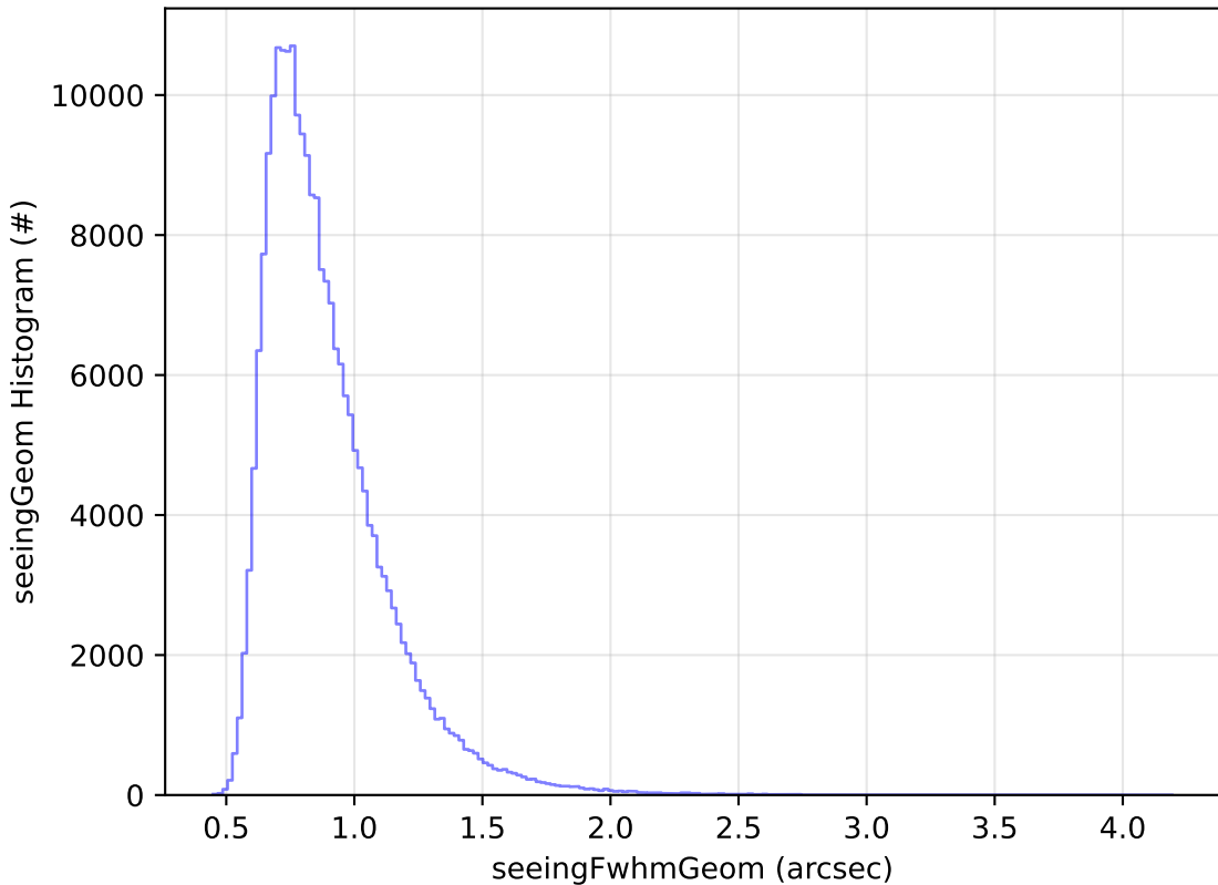
noroll_v3.4_10yrs Yr 1 all bands: seeingGeom Histogram
