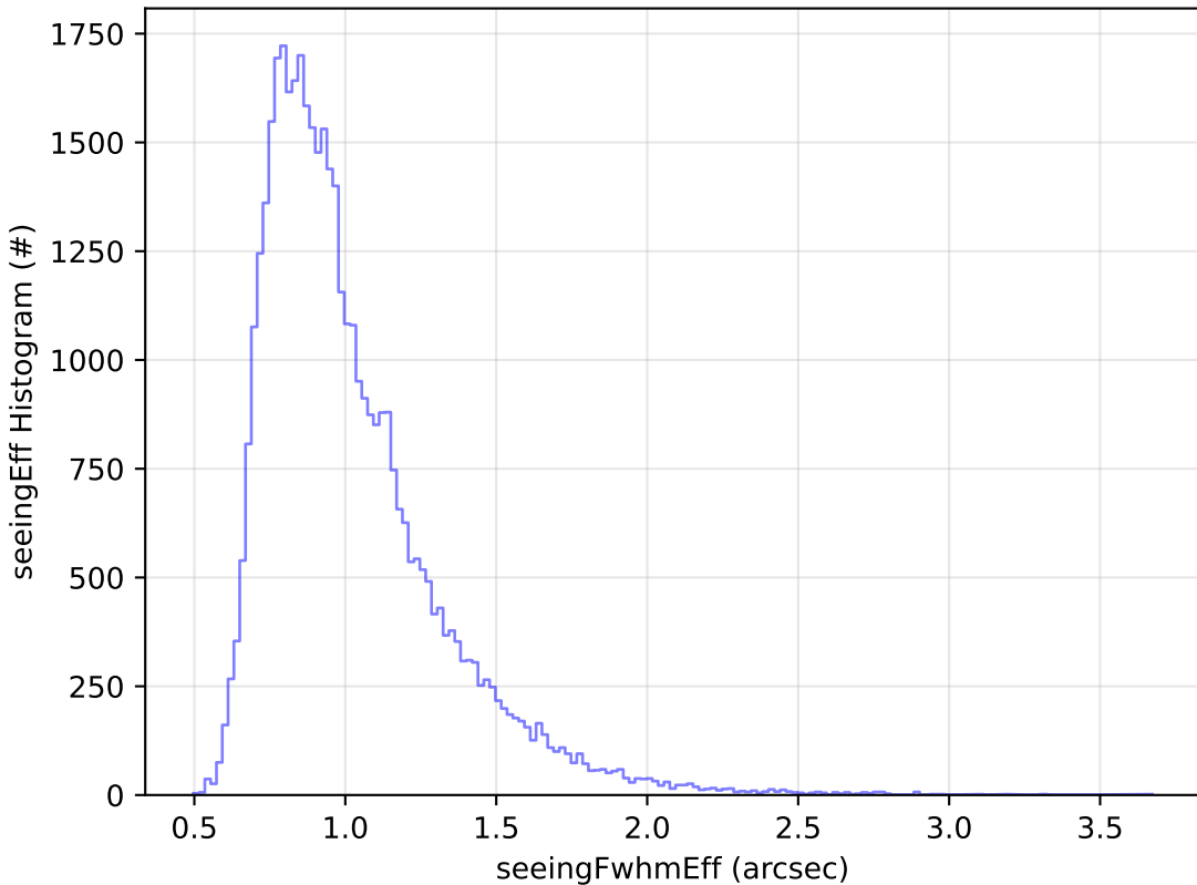
noroll_v3.4_10yrs Yr 1 z band: seeingEff Histogram
