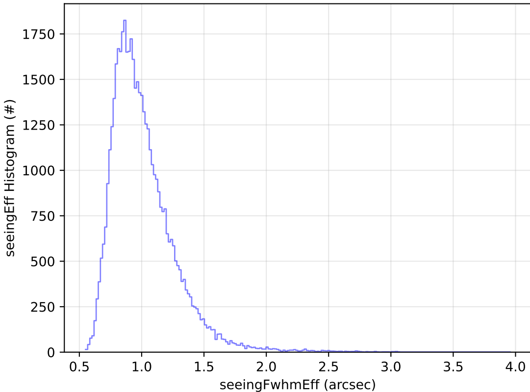
noroll_v3.4_10yrs Yr 1 y band: seeingEff Histogram
