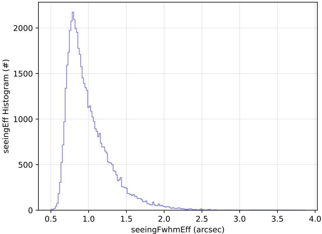
noroll_v3.4_10yrs Yr 1 r band: seeingEff Histogram
