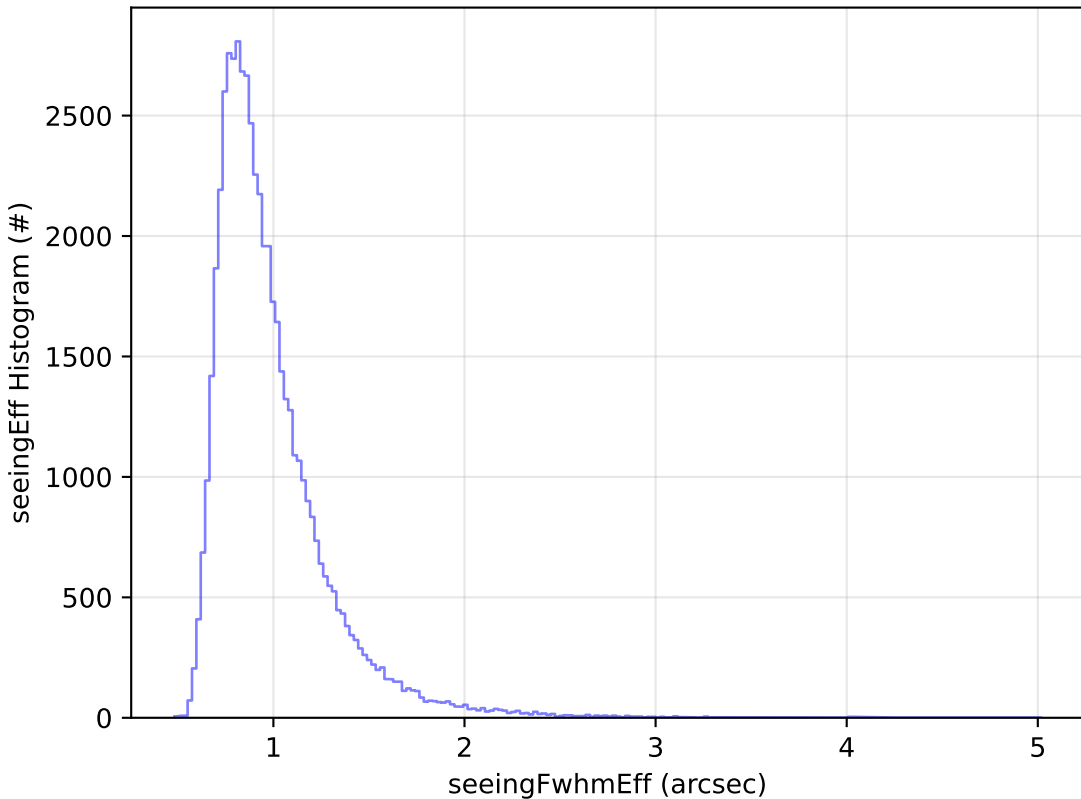
noroll_v3.4_10yrs Yr 1 i band: seeingEff Histogram
