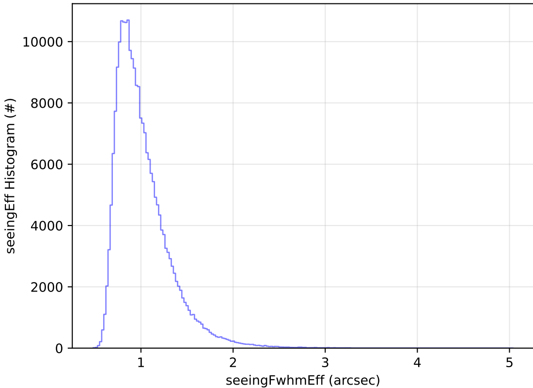
noroll_v3.4_10yrs Yr 1 all bands: seeingEff Histogram
