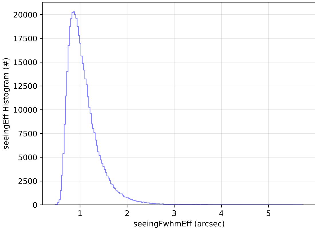
noroll_v3.4_10yrs WFD z band: seeingEff Histogram
