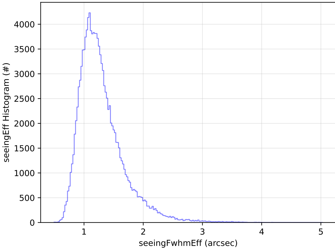
noroll_v3.4_10yrs WFD u band: seeingEff Histogram
