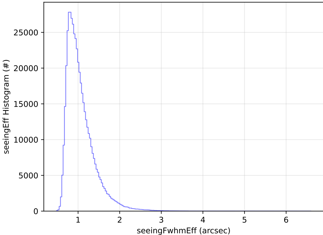
noroll_v3.4_10yrs WFD i band: seeingEff Histogram
