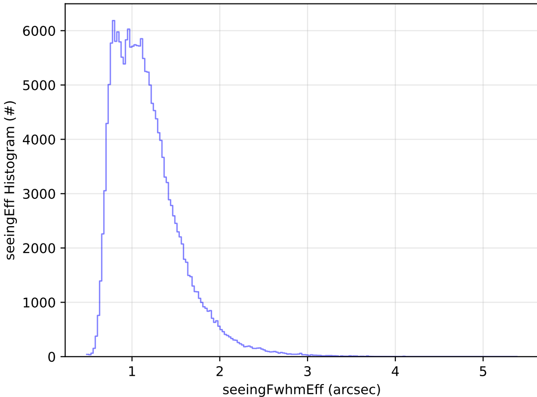
noroll_v3.4_10yrs WFD g band: seeingEff Histogram
