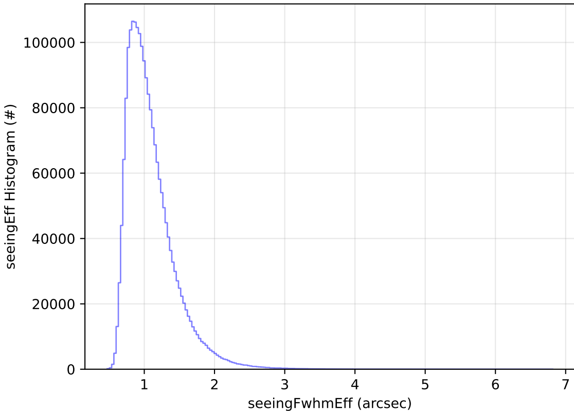
noroll_v3.4_10yrs WFD all bands: seeingEff Histogram
