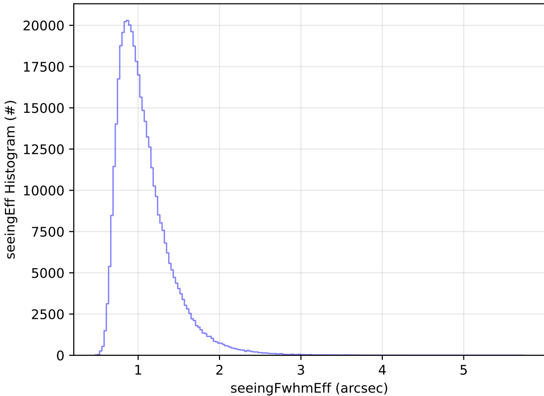
noroll_v3.4_10yrs All sky z band: seeingEff Histogram
