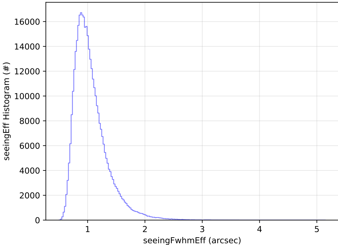
noroll_v3.4_10yrs All sky y band: seeingEff Histogram
