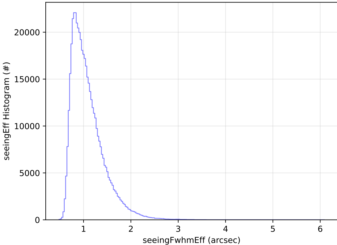
noroll_v3.4_10yrs All sky r band: seeingEff Histogram
