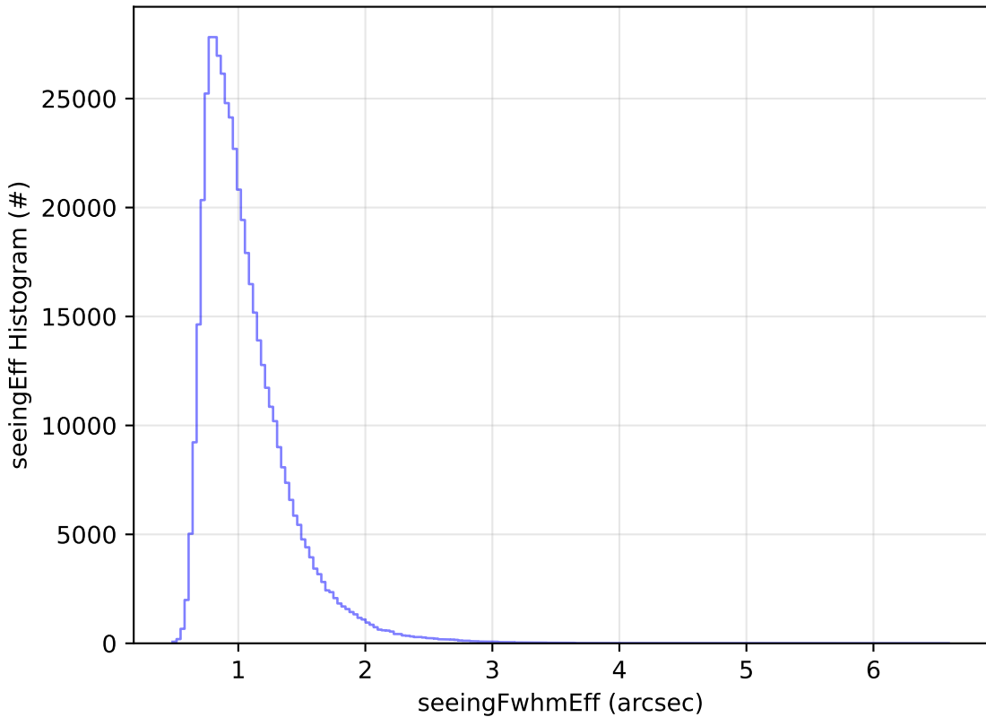
noroll_v3.4_10yrs All sky i band: seeingEff Histogram
