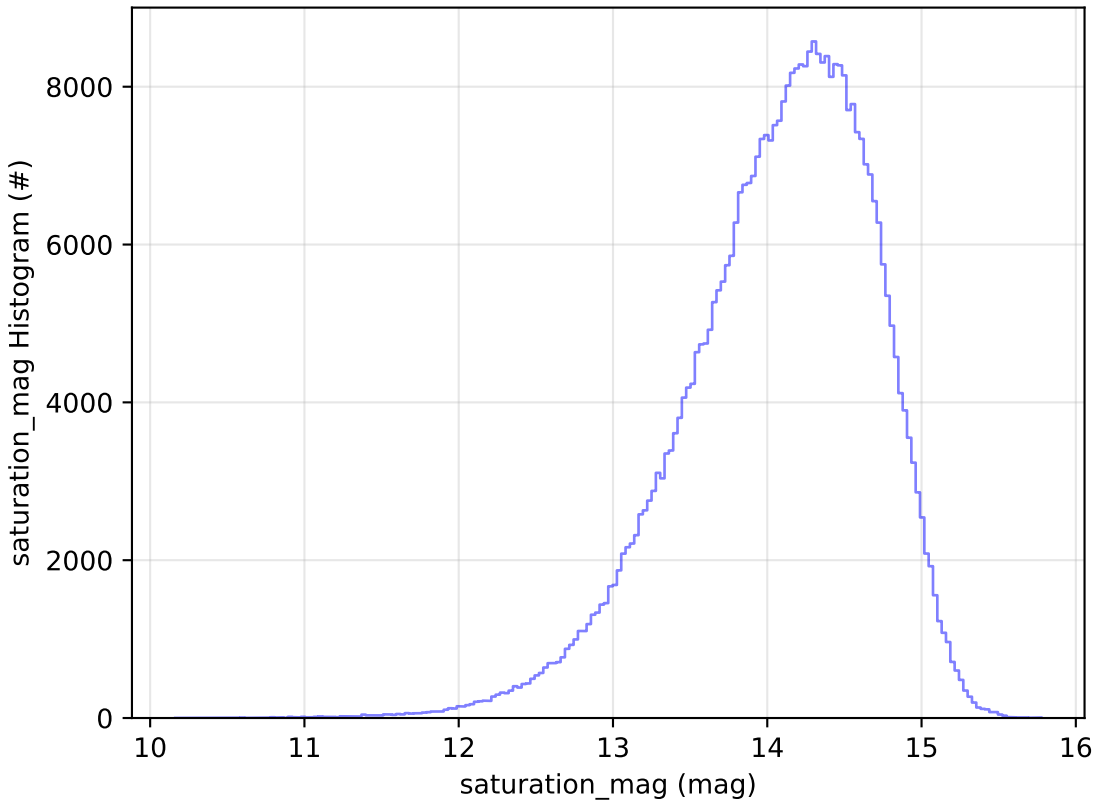
noroll_v3.4_10yrs WFD z band: saturation_mag Histogram
