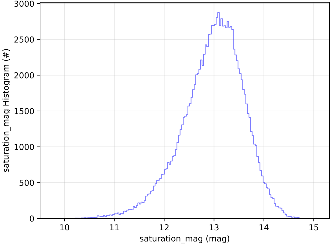
noroll_v3.4_10yrs WFD u band: saturation_mag Histogram
