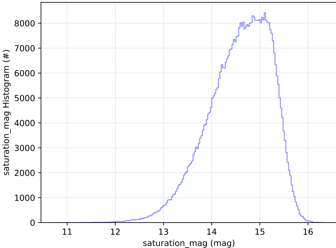
noroll_v3.4_10yrs WFD r band: saturation_mag Histogram
