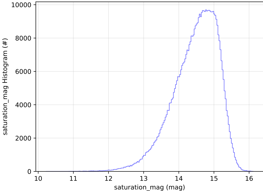
noroll_v3.4_10yrs WFD i band: saturation_mag Histogram
