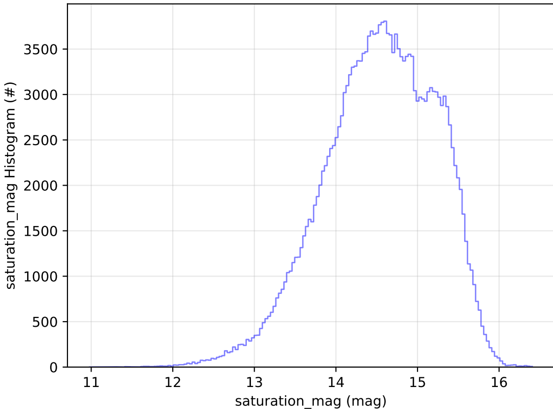
noroll_v3.4_10yrs WFD g band: saturation_mag Histogram
