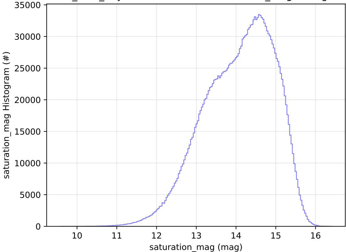
noroll_v3.4_10yrs WFD all bands: saturation_mag Histogram
