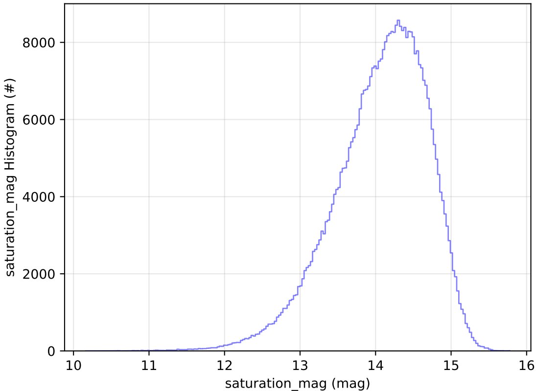
noroll_v3.4_10yrs All sky z band: saturation_mag Histogram
