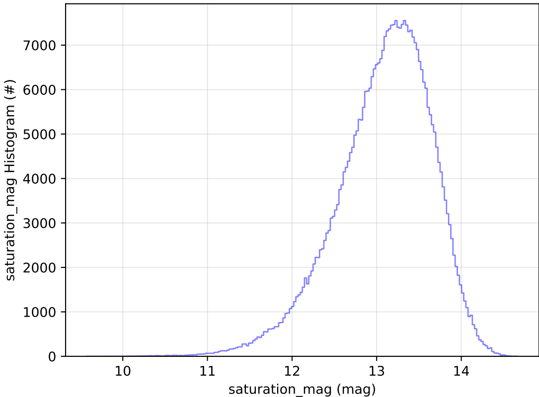
noroll_v3.4_10yrs All sky y band: saturation_mag Histogram
