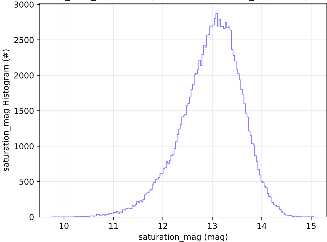
noroll_v3.4_10yrs All sky u band: saturation_mag Histogram
